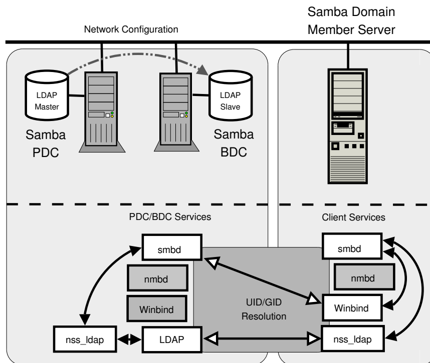
Figure 7.2. Samba Domain: Samba Member Server
